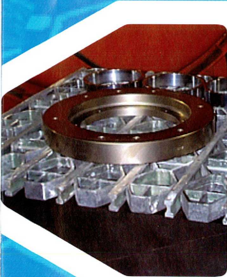
1.5" high POWER GRID™ used in a nickel brazing process
