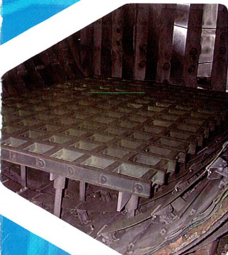
2" high POWER GRID™ used in vacuum annealing
